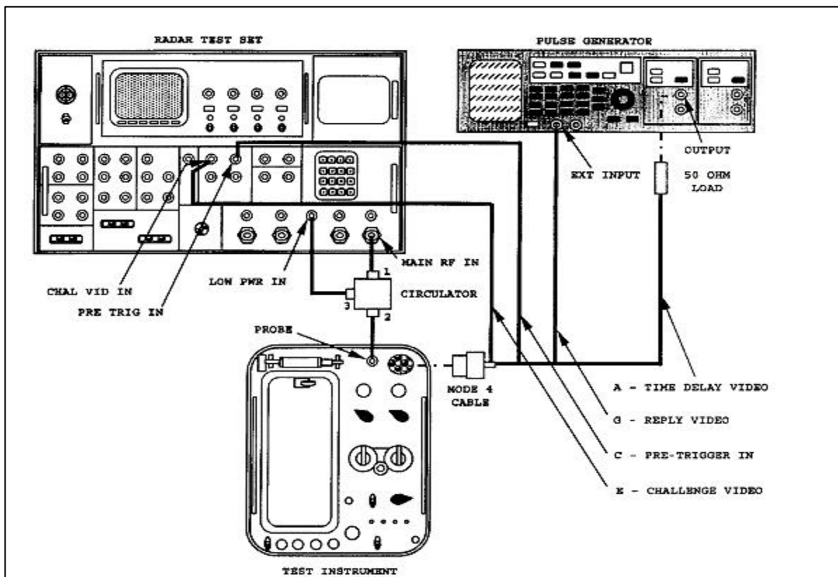
Mode 4 Connector Pin Out
